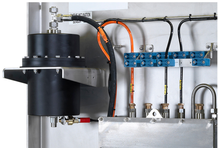
Flange-mounted 6-liter Basic series compensator
